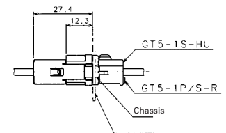
Assembly Diagram (1:1)
