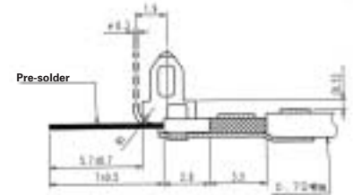
◆ Completed Termination Cross Section
