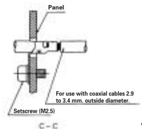
◆ Attachment Diagram
