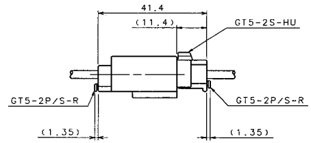
◆ Diagram of Mated Connector in Use
